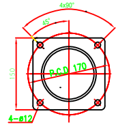
EXHAUST ELBOW FLANGE(2/1)
