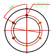
CRANK SHAFT PULLEY(2/1)
