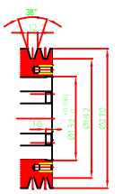
CRANK SHAFT PULLEY(2/1)
